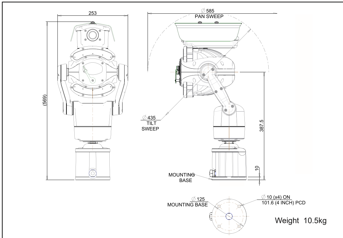
Dual View Dimintions & Predator Thermal (up to 35mm lens) with LED array and built in thermal encoder
